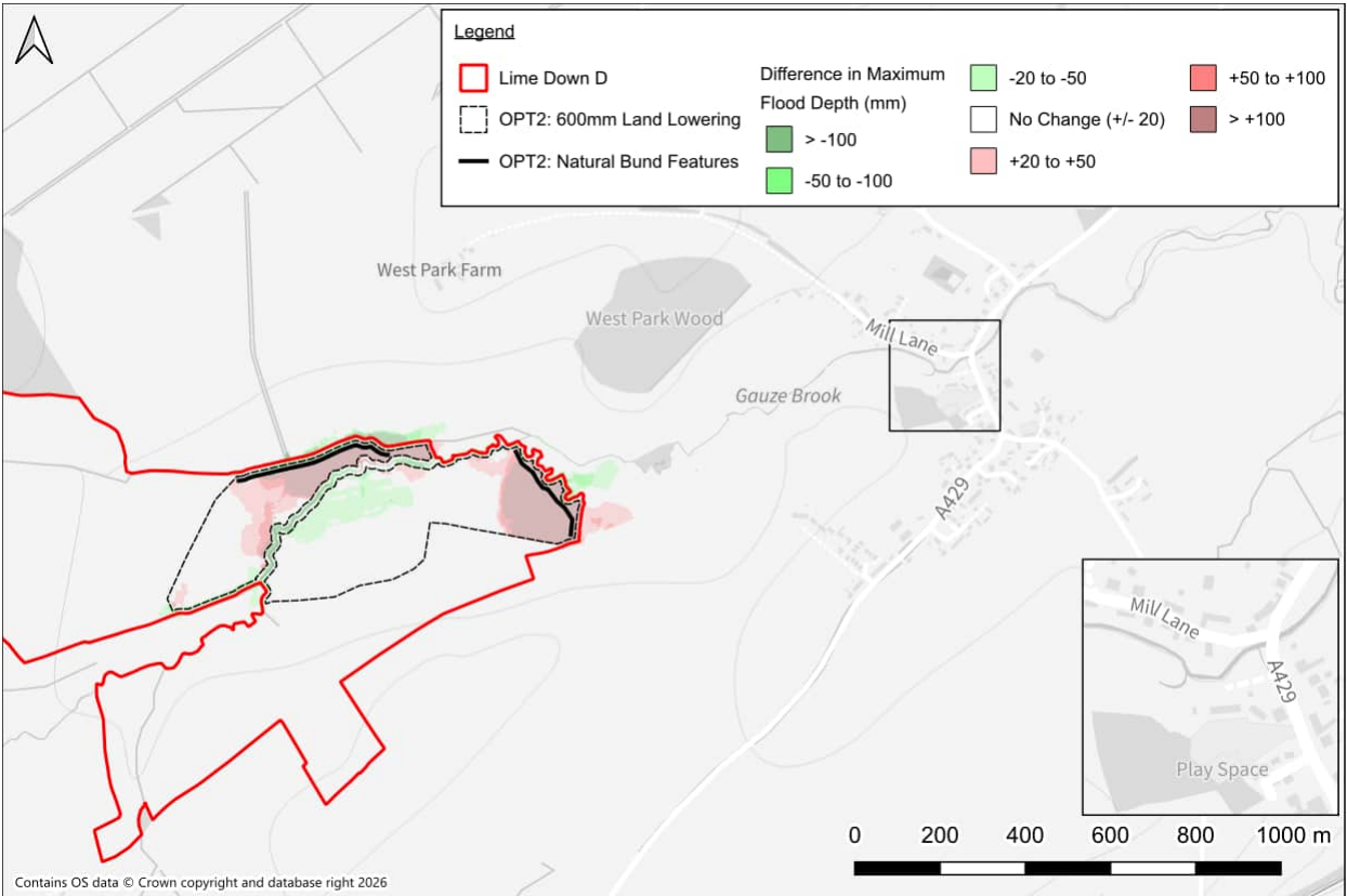
Figure 11: OPT2 difference in maximum flood depths – 1% AEP +39%CC fluvial event
