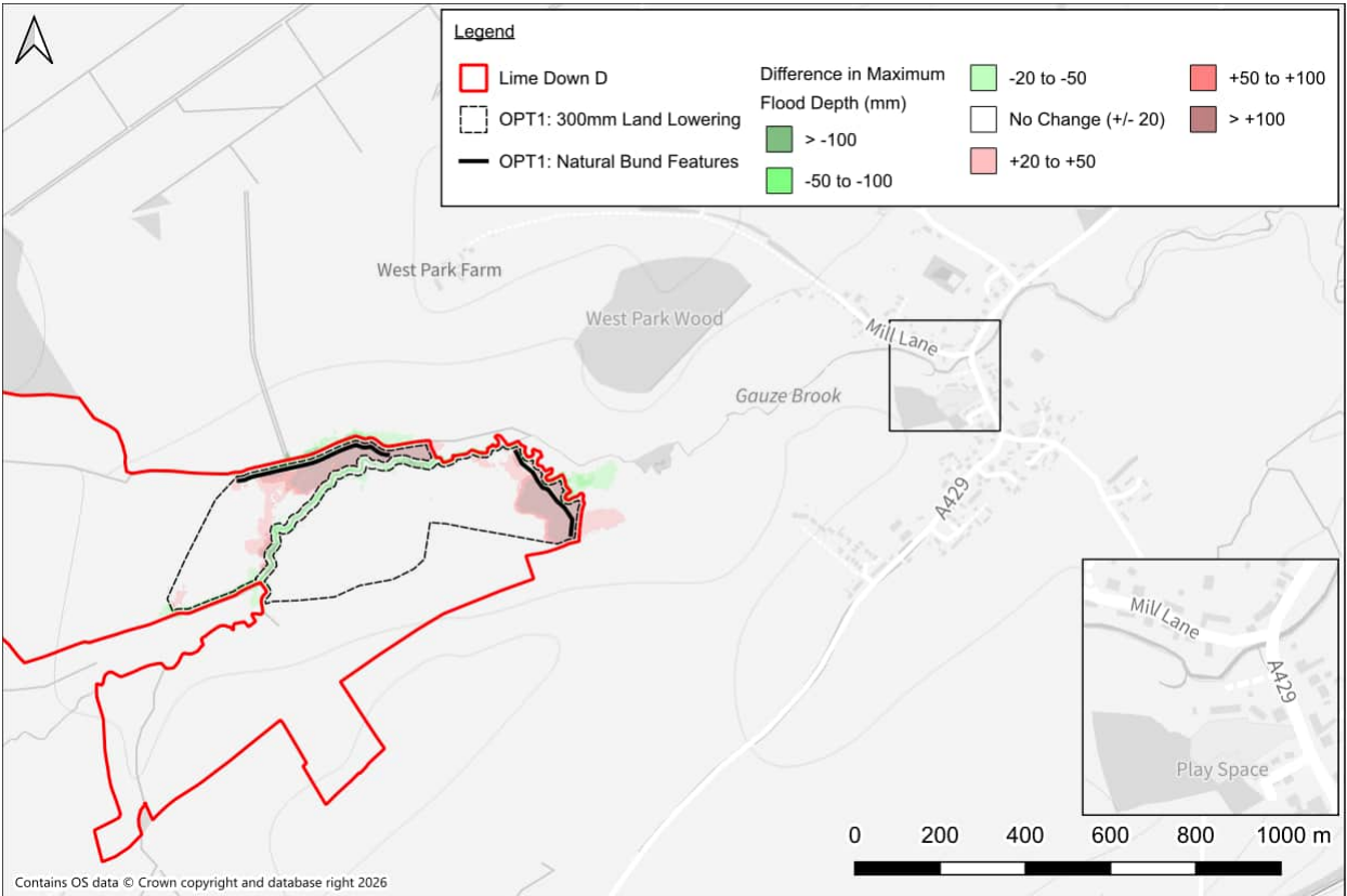
Figure 10: OPT1 difference in maximum flood depths – 1% AEP +39%CC fluvial event
