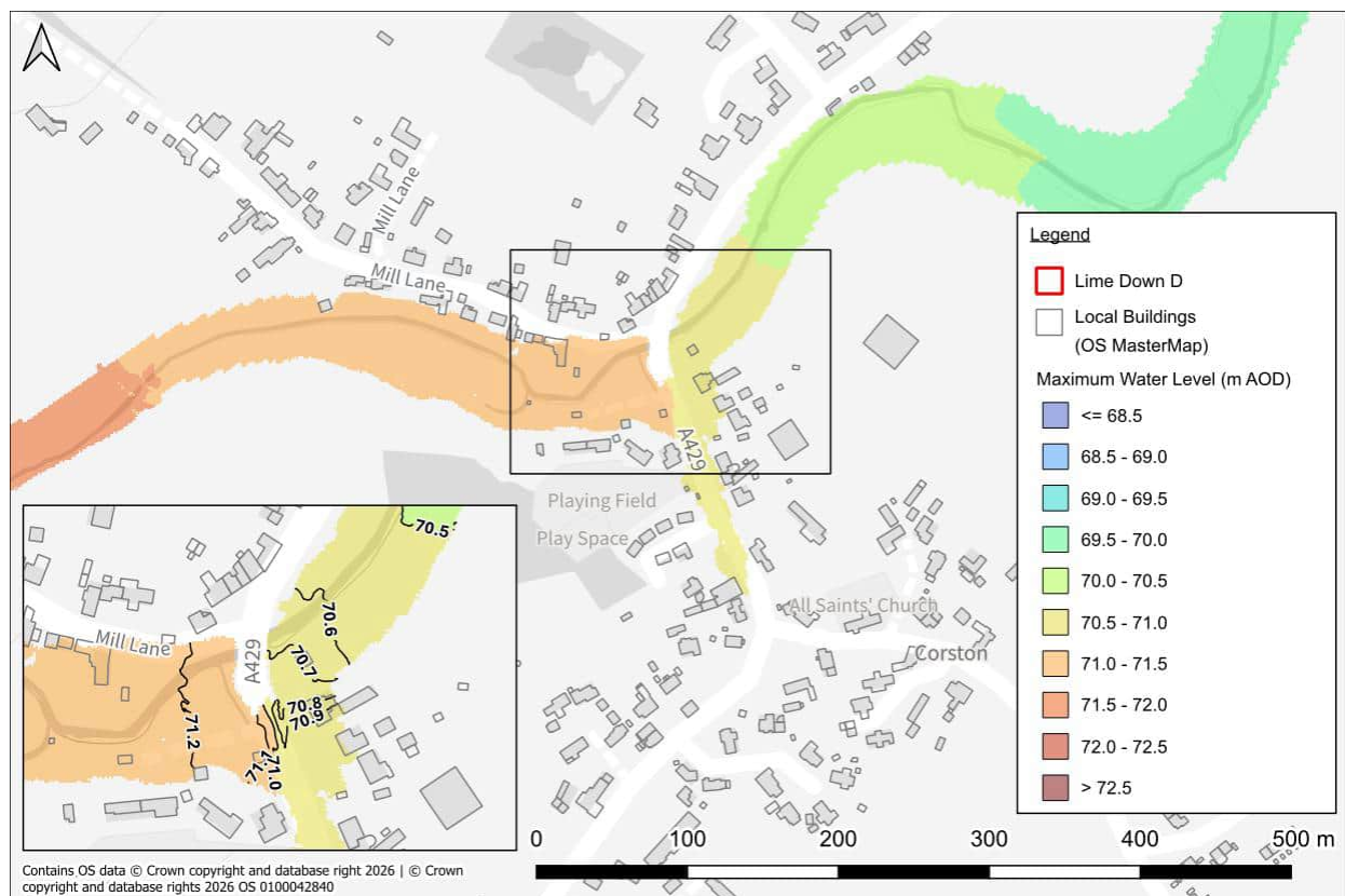
Figure 12: Maximum water levels through Corston, 1% AEP +39%CC fluvial event, baseline scenario
